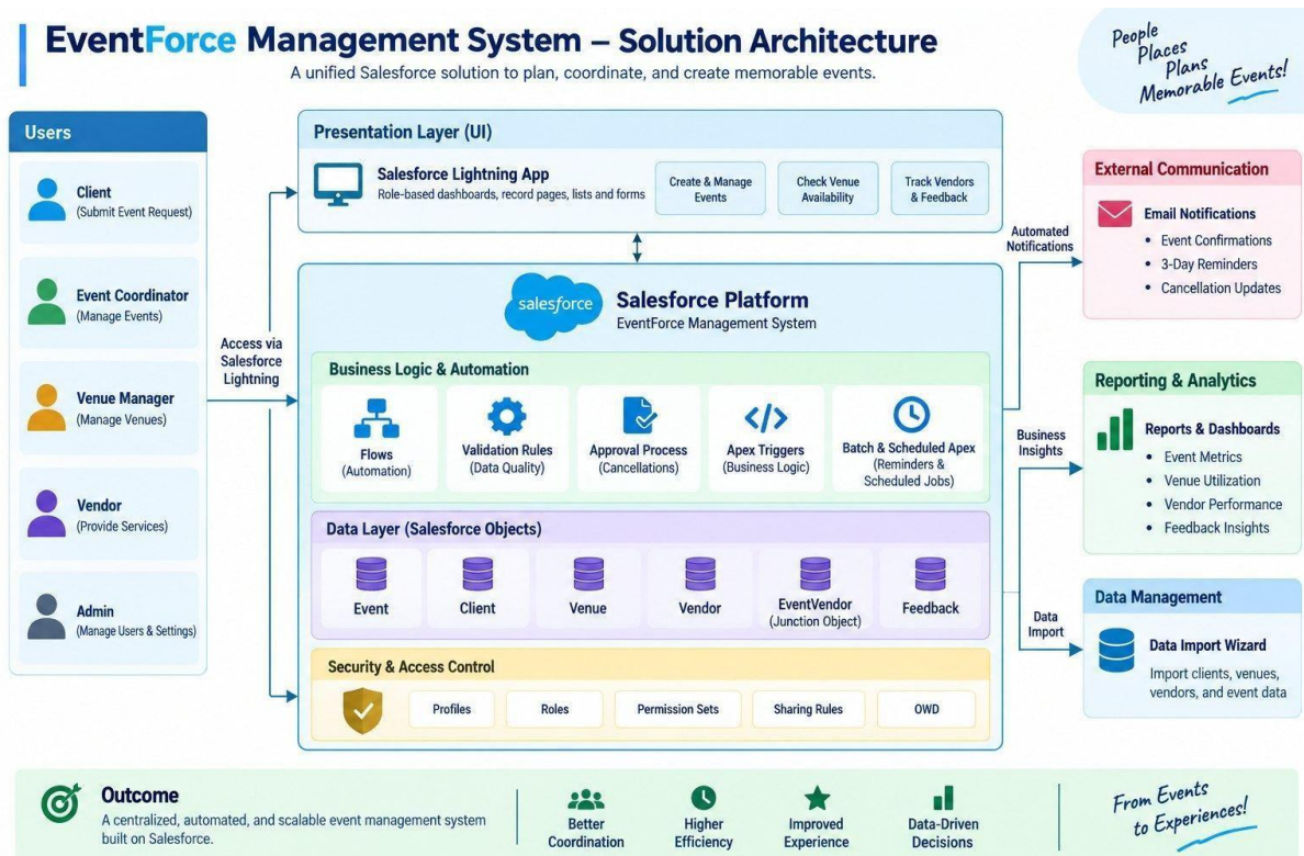
Figure 4.2 – Solution Architecture
